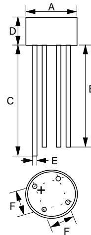
Dimensions in millimeters(1mm =0.0394")
